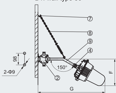
B1: wall type 30°
