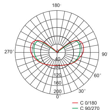
Luminous intensity distribution (cd/1000lm)
