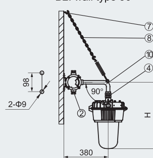
B2: wall type 90°
