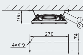
X: ceiling type
